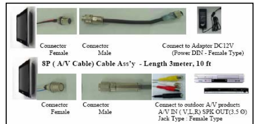
Waterproof Connectors
