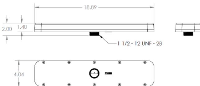
Figure 2. Product Dimensions
